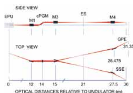
Figure 2. Optical layout of the beamline: EPU is an undulator (light source); M1, M3, M4 are mirrors, ES is an exit slit and cPGM is a monochromator.
